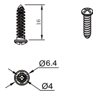
Countersunk cross topping screw M4*16
