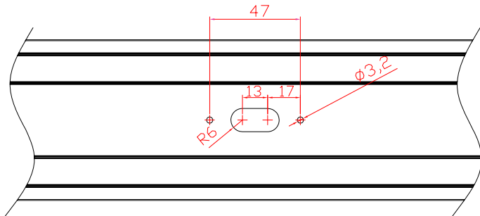
① : T10 panels connection holes
