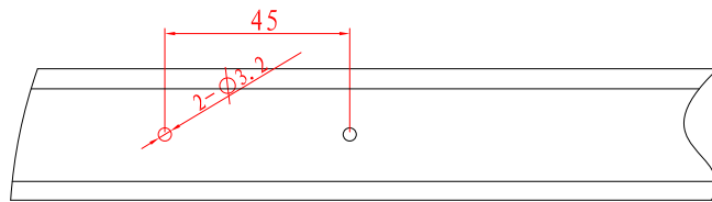
③ : T3 panels connection holes
