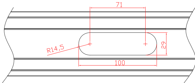
② : wires passing hole
