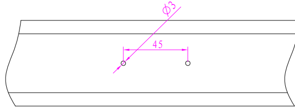
① : T8 panels connection holes
