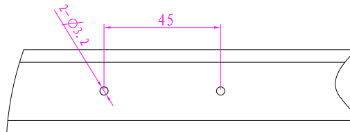
③ : T3 panels connection holes
