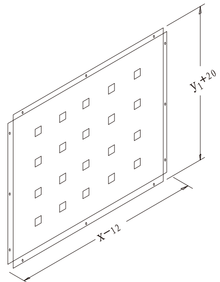
Metal sheet
