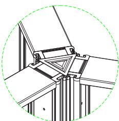
120° 3 ways connection
