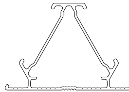
120° 2 ways connection pole 3467#
