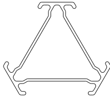
120° 3 ways connection pole 3175#
