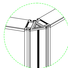
120° 2 ways connection
